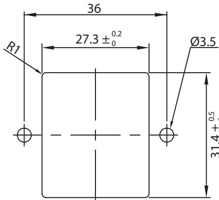
PANEL CUTOUT
